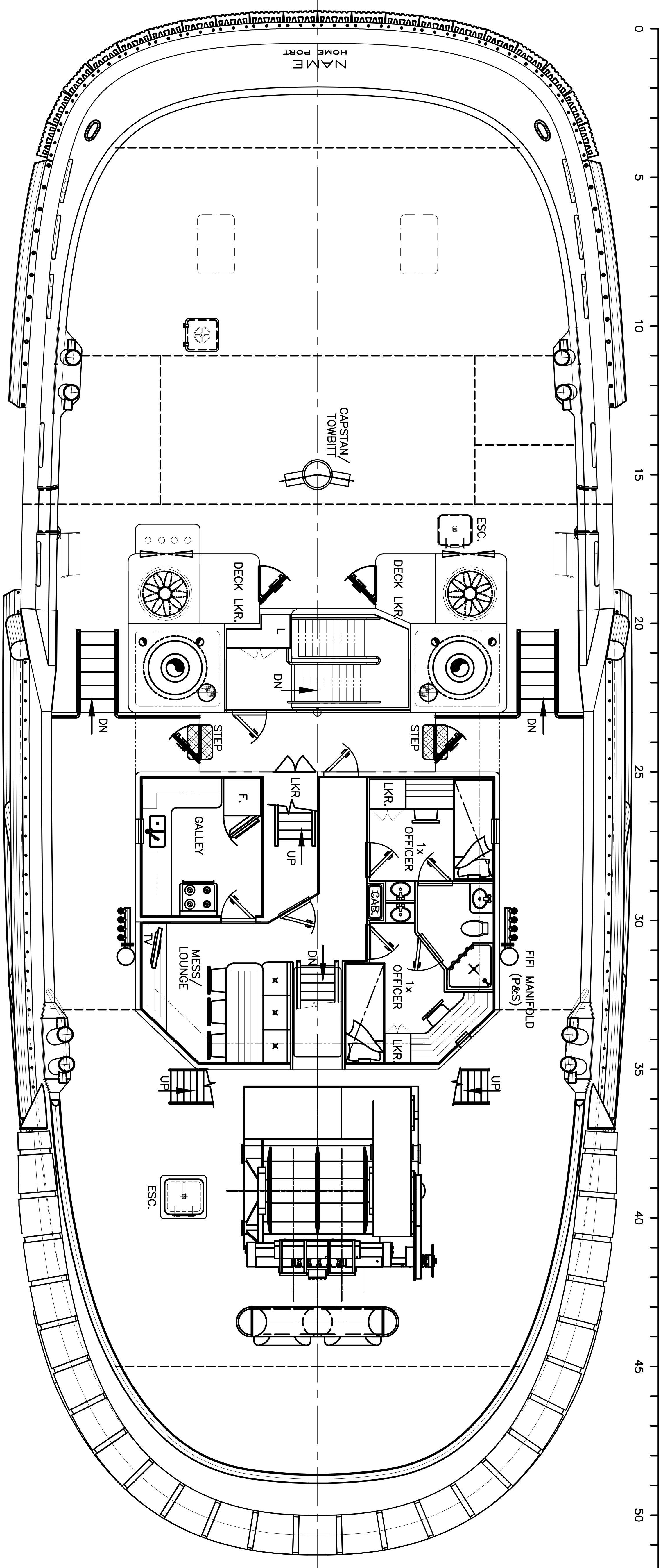
BRIDGE DECK PLAN
